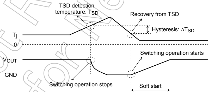
Figure 6 Thermal Shutdown Operation
