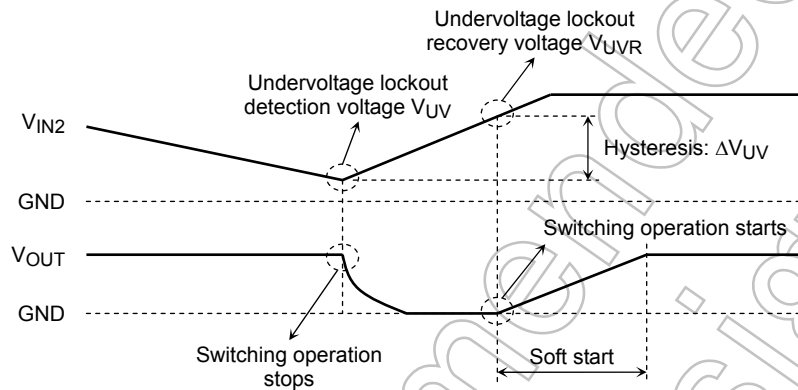
Figure 5 Undervoltage Lockout Operation
