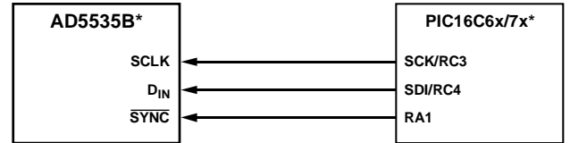
Figure 18. AD5535B-to-PIC16C6x/7x Interface
