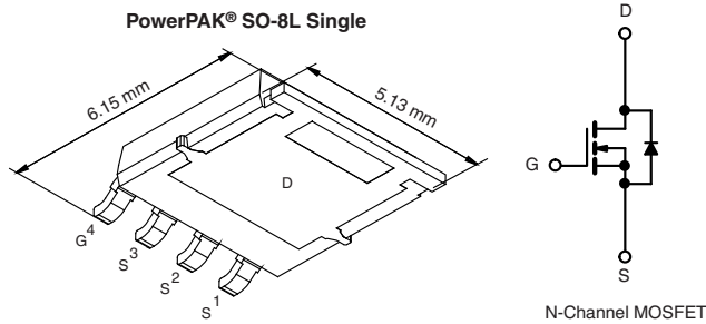
N-Channel MOSFET
