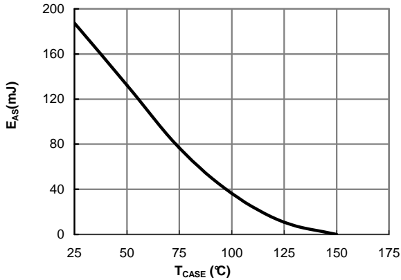
Figure 12: Avalanche energy
